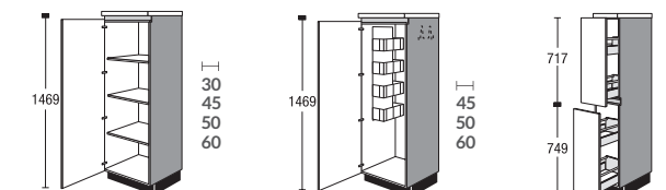
CS...151 HE Highboard Highboard CS...151 HEB Highboard à balais Highboard als werkkast CSA...151 HA Highboard Highboard
